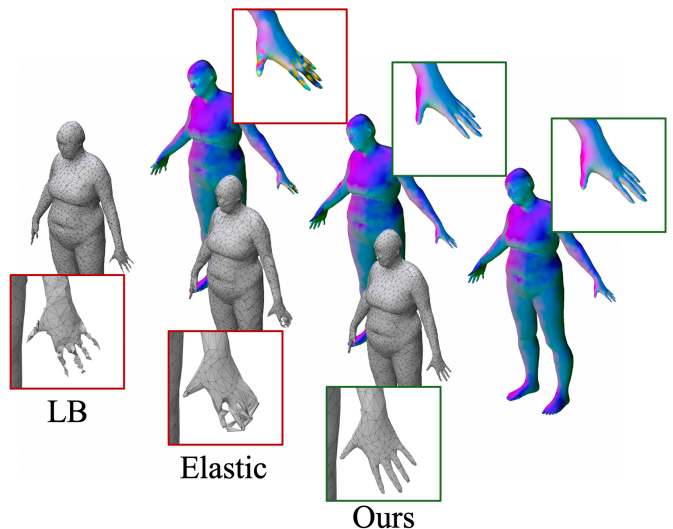
Figure 6. Qualitative Results on FAUST. Comparison of ULRSSM in the LBO basis, elastic basis (orthogonalized) and in the proposed hybrid basis. We show both normal and vertex position transfers. The hybrid basis (ours) yields the most accurate mapping, particularly noticeable in the hand region.
