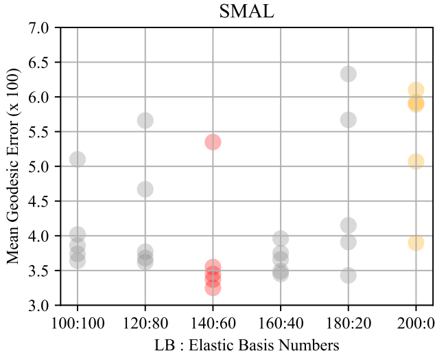
Figure 15. Hybrid ULRSSM is evaluated on SMAL using a varying ratio of LBO and elastic eigenfunctions. Our basis ratio can be observed in red, with the baseline pure LBO implementation in yellow.
