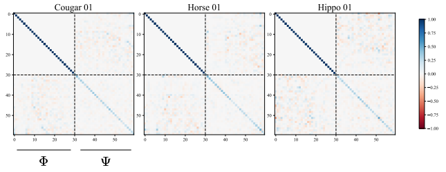
Figure 8. Matrix of inner product between hybrid basis M_{k_{\text{total}}} = [\Phi \Psi]^T M [\Phi \Psi] , with k_{\text{total}} = 30 + 30 . We show the heatmap of the resulting matrix from three animal shapes of the SMAL dataset.
