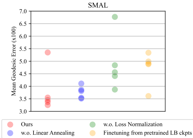
Figure 17. Ablation study of optimization strategies using Hybrid ULRSSM on SMAL. Five random runs are shown for each training setting.
