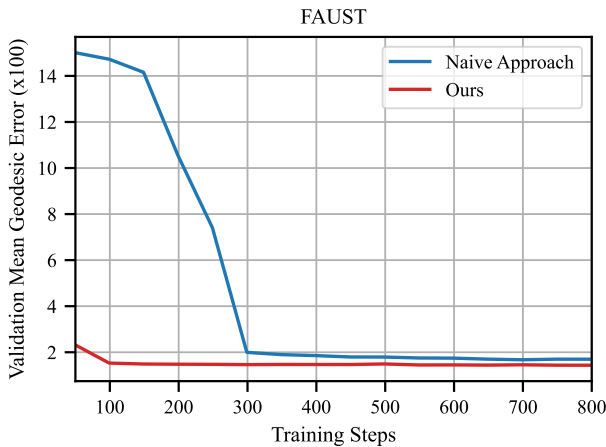
Figure 13. Ablation study concerning separate optimization of the block matrix on FAUST with Hybrid ULRSSM. The y-axis depicts validation error, while the x-axis shows training steps. Separating the optimization problems primarily leads to faster convergence.
