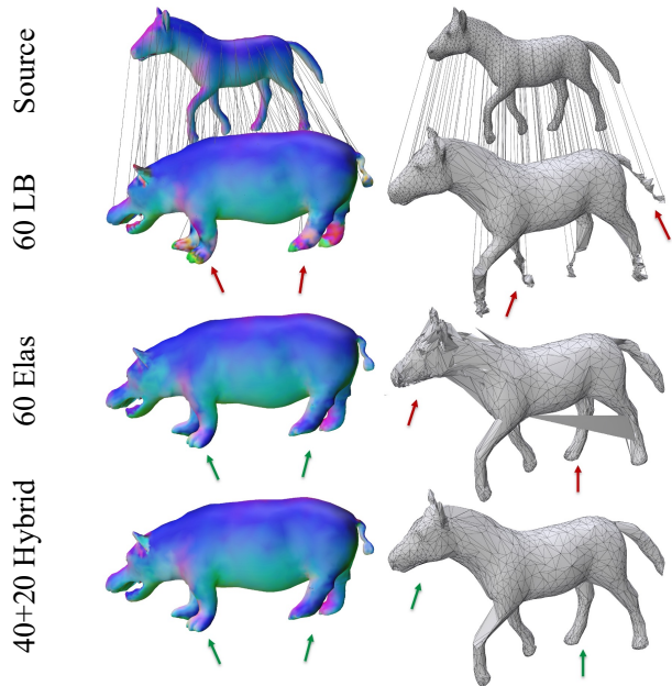
Figure 3. Comparison of correspondence visualizations by transferring normal colors (left) and vertex positions (right) from the source to the target shape. We examine the results from LB, Elastic, and Hybrid basis functions by encoding and recovering ground truth correspondences through functional map representations at a spectral resolution of k = 60 . Additional results at a spectral resolution of k = 200 are provided in the supplementary.
